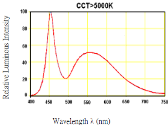
Fig.5 IF-Ta
