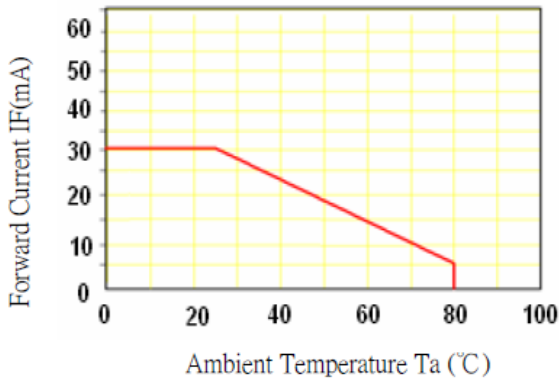
Fig.5 IF-Ta
