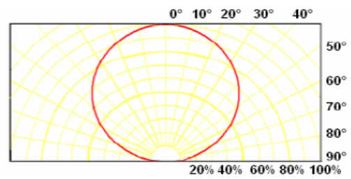
Directive Characteristics (Ta=25°C)
