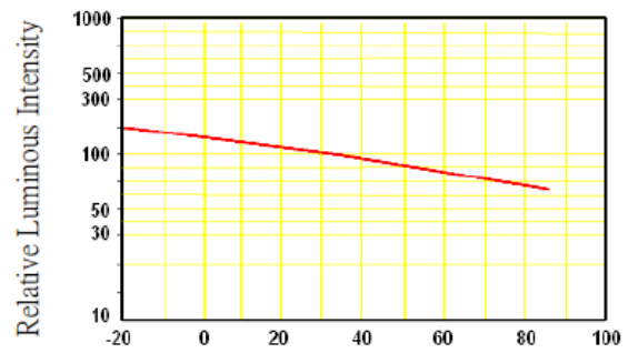
Fig.4 Relative Luminous Intensity-Ta
